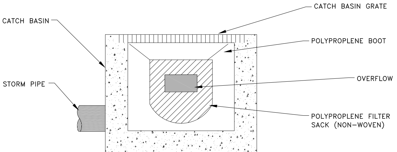
NON-WOVEN POLYPROPYLENE SACK
