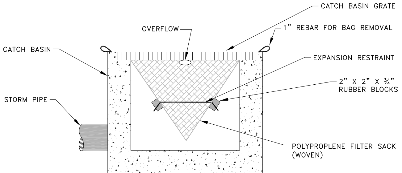
WOVEN POLYPROPYLENE SACK
