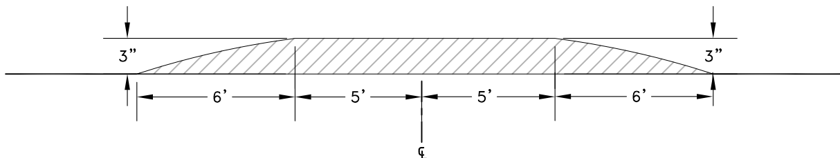
PARABOLIC CROWN SECTION A-A
