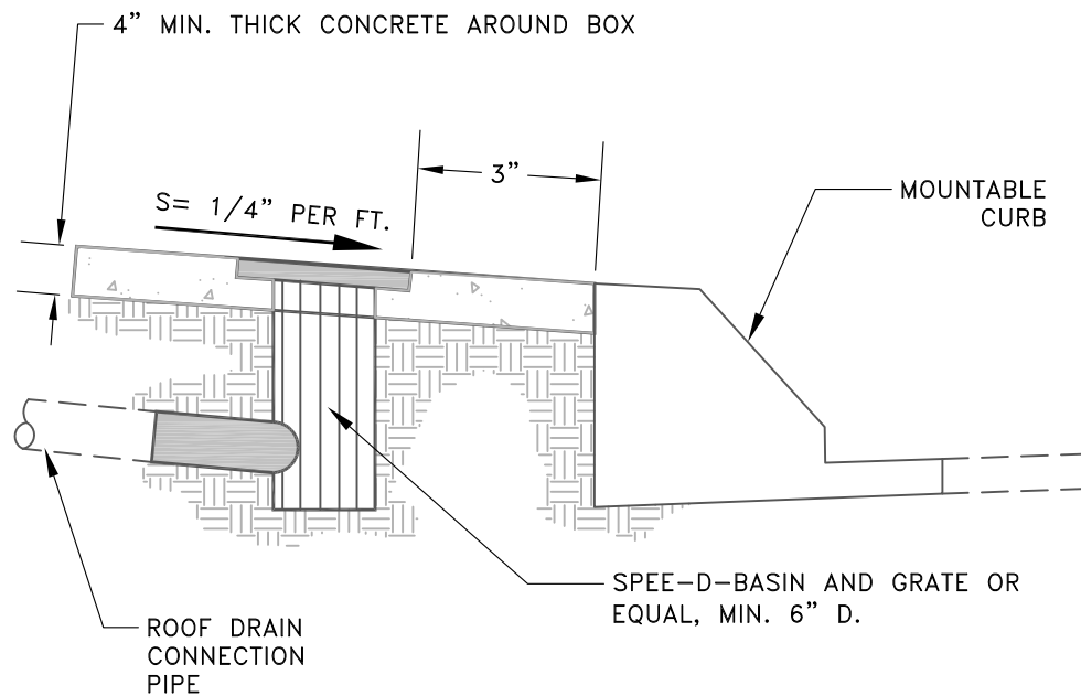
SIDE VIEW
